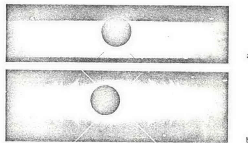
Figure 2. Diffraction patterns of \text{Cd}_3\text{As}_2 in gas-loaded diamond-anvil pressure unit: (a) tetragonal, ~20 kbar; (b) trigonal, >50 kbar.
